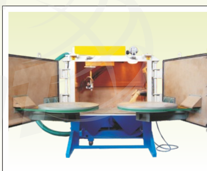
Automatic Blast Cabinet for Glass Mould Cleaning with dual Door Mounted Turn Tables for increase production & Nozzle Reciprocation
