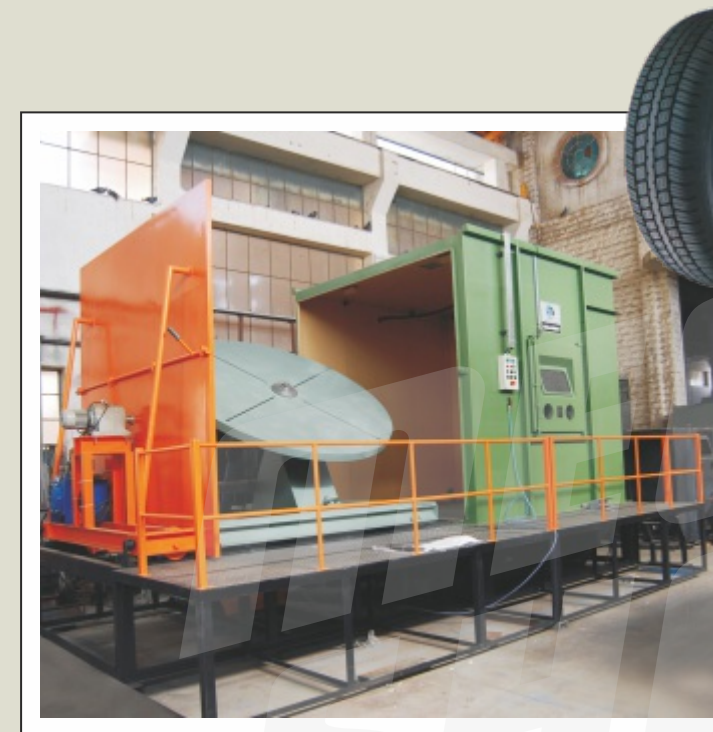
Blast Cabinet for cleaning of Tyre Molds. It features tilting turntable, trolley with motorised winch. Gun movement with rack pinion arrangement to cover mold.
