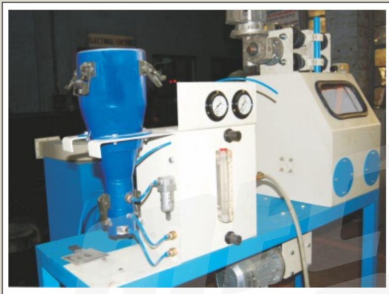
'MECSHOT' Spray Blasting Equipment to spray Micro Blast and coat Alumina Powder of 5 & 0.5 Micron particle size on SS-440C pins of Hardness 54 Rc and size 8mm dia x 100mm length to achieve the high temperature resistance coatings.
